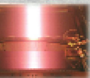
High heat flux test of protecting armour tiles
