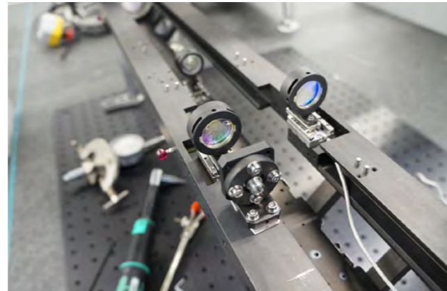
Prototype of the IVVS Measurement System probe, during assembly. ©F4E
